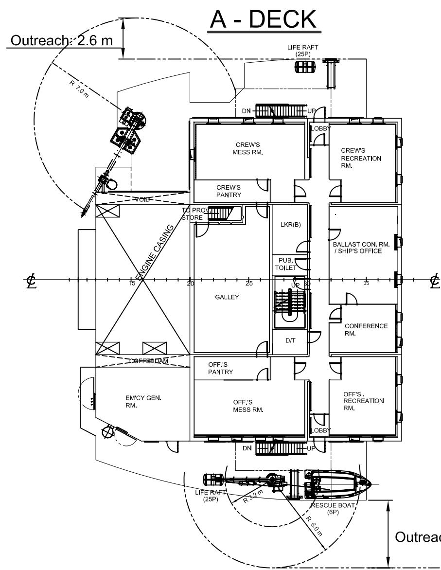
A - DECK
