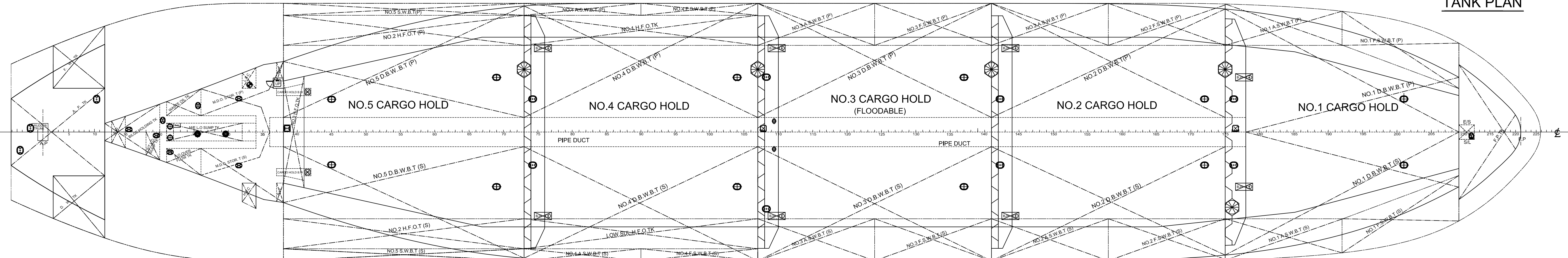
TANK PLAN
