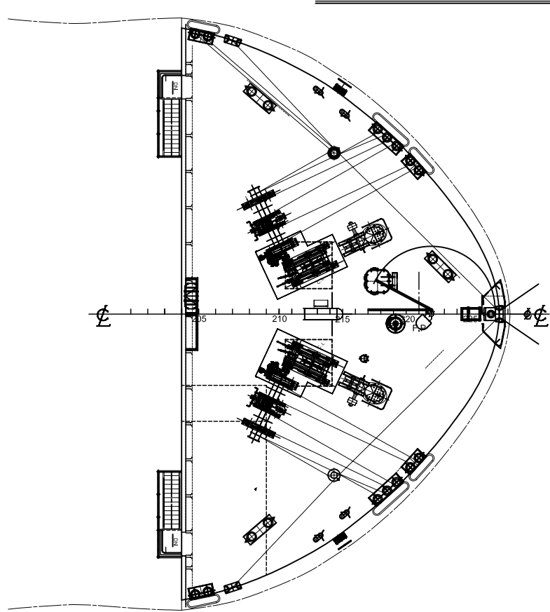
F'CLE DECK
