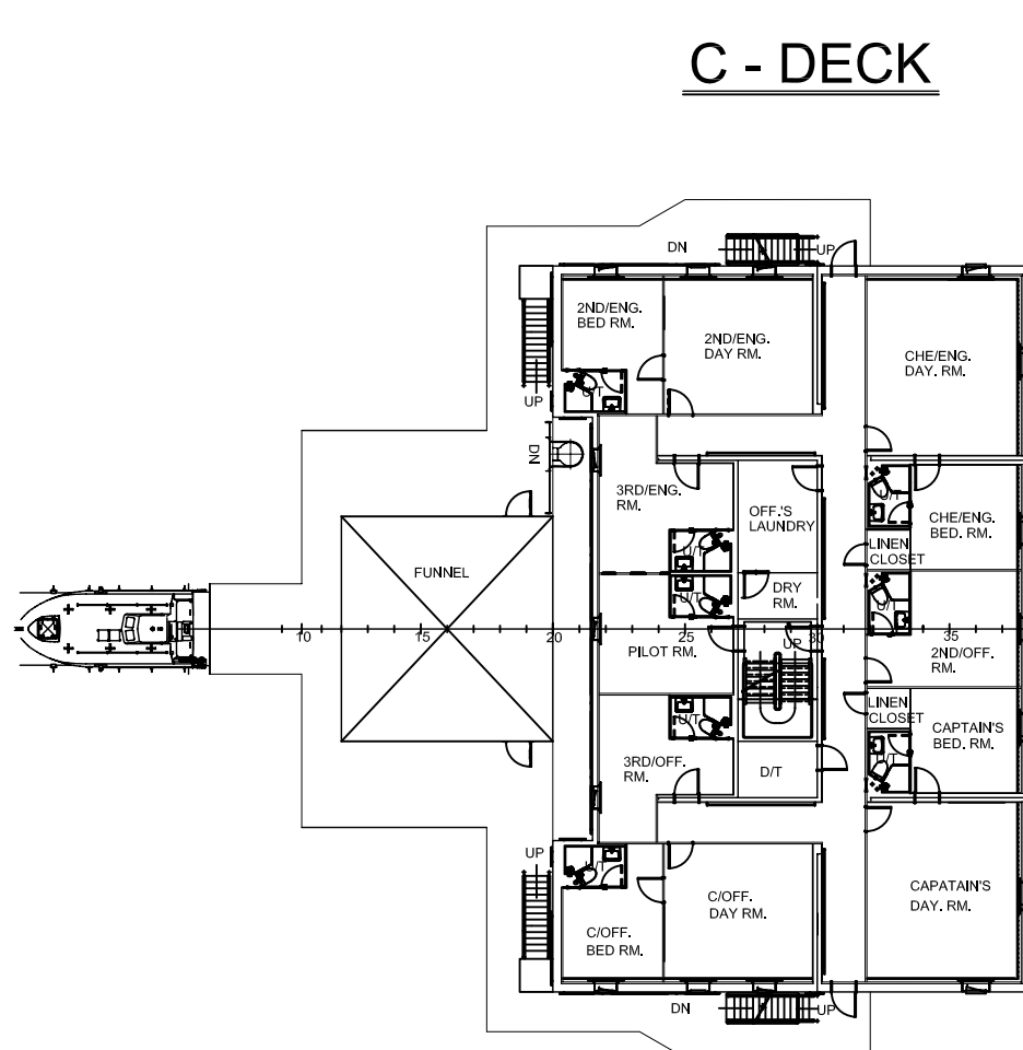
C - DECK
