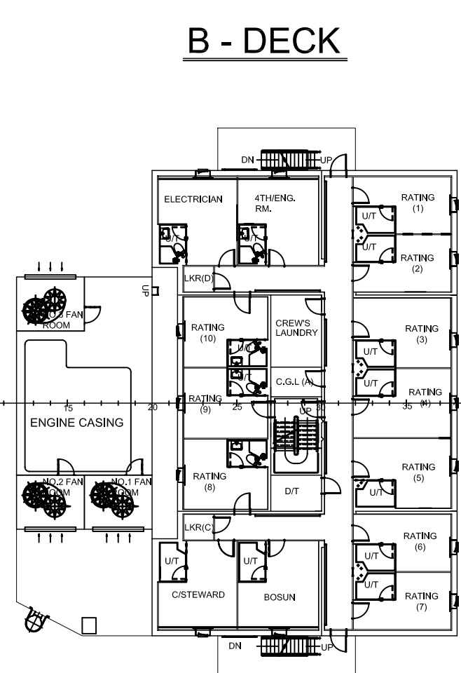
B - DECK
