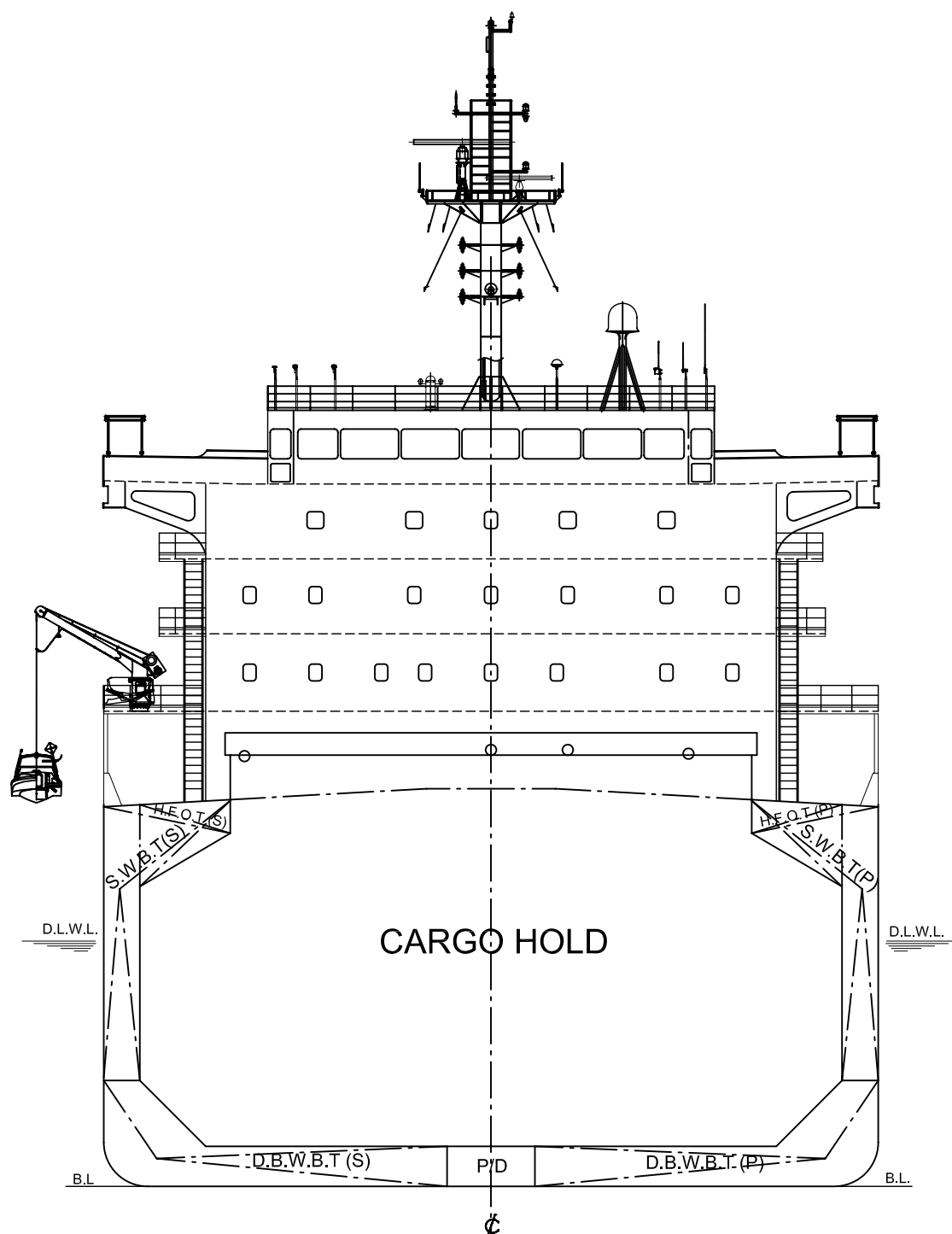
MIDSHIP SECTION (LOOKING AFT)
